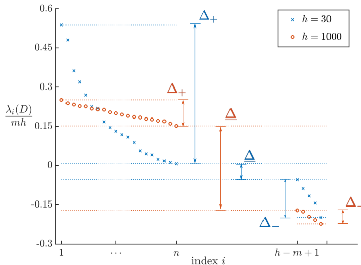
Figure 4: Scaled eigenvalues of the imbalance matrix D and the corresponding scaled imbalance quantities \frac{1}{mh} \Delta_+, \frac{1}{mh} \Delta_-, \frac{1}{mh} \underline{\Delta} under random initialization, the scaling factor is omitted in the plot annotation for simplicity. When the network has small width h = 30 , spectrum spreads \Delta_+, \Delta_- are larger compare to the level of imbalance \underline{\Delta} . large width h = 1000 network shows the opposite.
