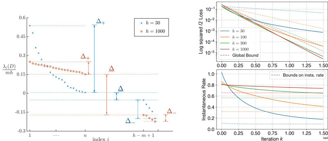
Figure 2: (Left): Scaled eigenvalues of the imbalance matrix D and the corresponding scaled imbalance quantities \frac{1}{mh}\Delta_+ , \frac{1}{mh}\Delta_- , \frac{1}{mh}\underline{\Delta} under random initialization, the scaling factor is omitted in the plot annotation for simplicity.
