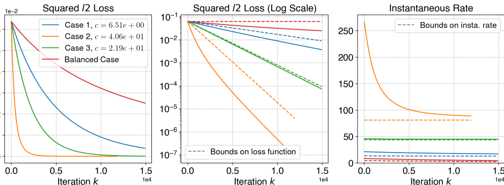
Figure 3: Convergence of gradient descent on linear networks with different initial imbalance matrices. We plot the loss function \mathcal{L} on the left (Regular scale) and the middle (Log scale) figure. The instantaneous rate -\dot{\mathcal{L}}/\mathcal{L} is shown on the right figure. The dashed line on the middle plot shows the bound on loss function by Theorem 3. Lastly, the dashed line on the right plot shows the lower bound by Proposition 1.
