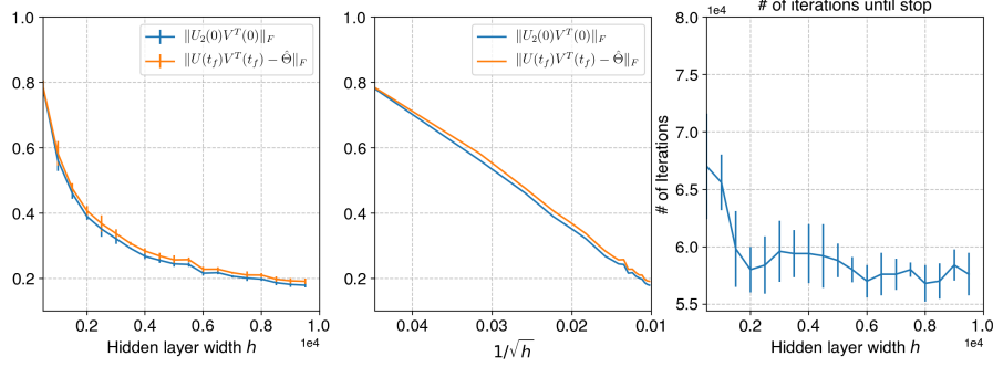
Figure 7: Implicit bias of wide single-hidden-layer linear network under random initialization. The line is plotting the average over 5 runs for each h , and the error bar shows the standard deviation. The gradient descent stops at iteration t_f .
