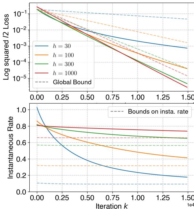
Figure 5: Gradient descent on \mathcal{L} = \frac{1}{2} \left\| Y - \frac{1}{\sqrt{mh}} UV^T \right\|_F^2 .
