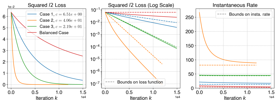
Figure 6: Convergence of gradient descent on linear networks with different initial imbalance matrices. We plot the loss function \mathcal{L} on the left (Regular scale) and the middle (Log scale) figure. The instantaneous rate -\dot{\mathcal{L}}/\mathcal{L} is shown on the right figure. The dashed line on the middle plot shows the bound on loss function by Theorem 3. Lastly, the dashed line on the right plot shows the lower bound by Proposition 1.
